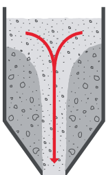
Funnel flow: reduced storage volume and segregation
