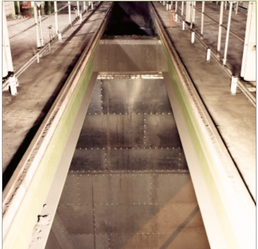
KALEN lining installed in a large German coal-fired power station. The material in the bunker is fine coal.
